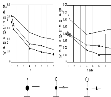
Fig4 The maximum displacements of the lower lumped mass decrease with increasing R factor of the plastic
