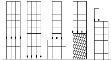
Fig 1. Vertically irregular buildings and locations of the weak storey.
